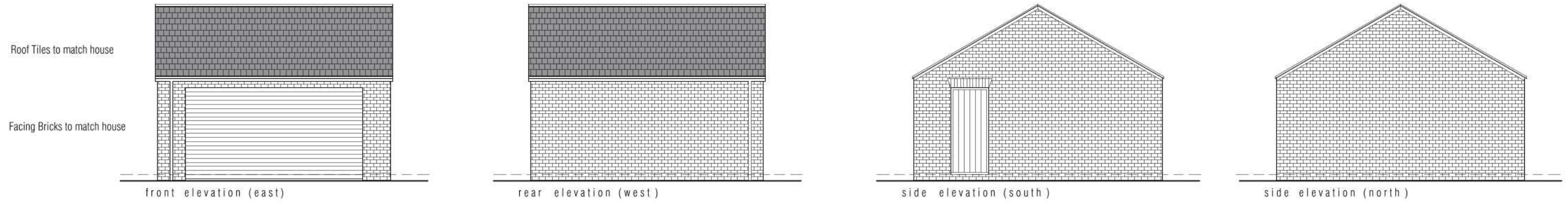
elevations as proposed 1:100 scale
