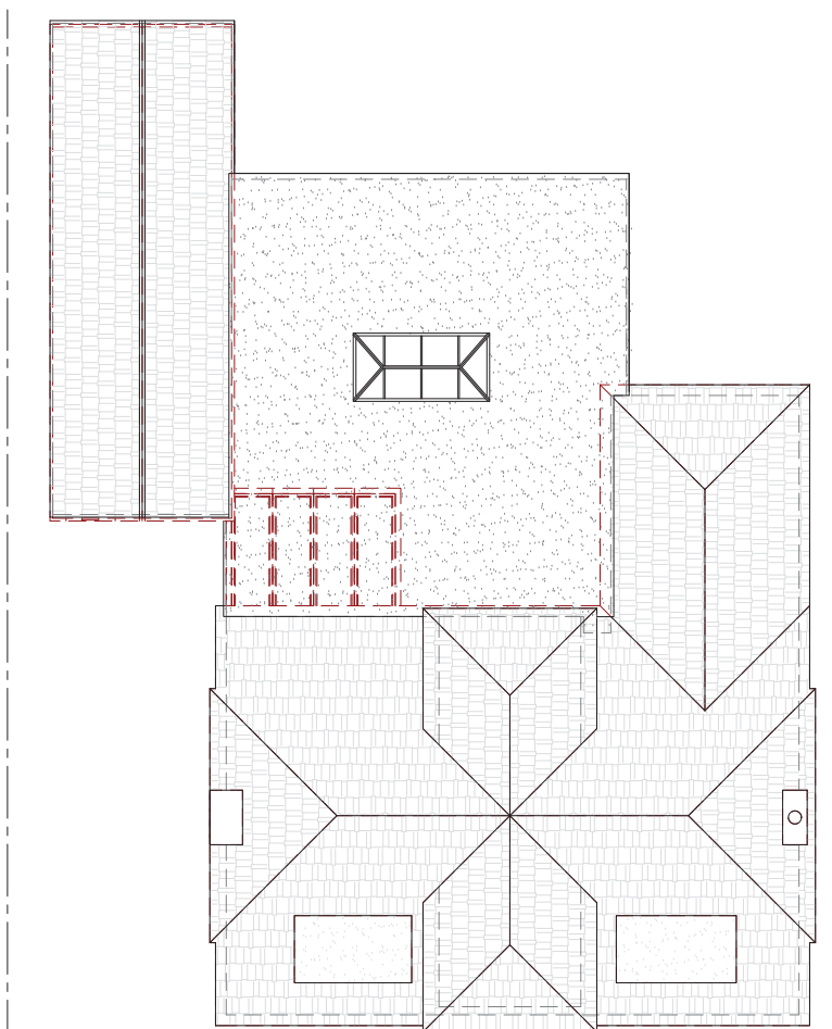
Proposed Roof Plan Scale 1:50
