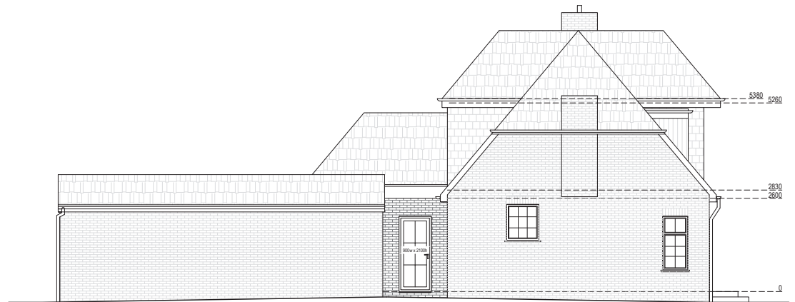
Proposed West Elevation Scale 1:50
