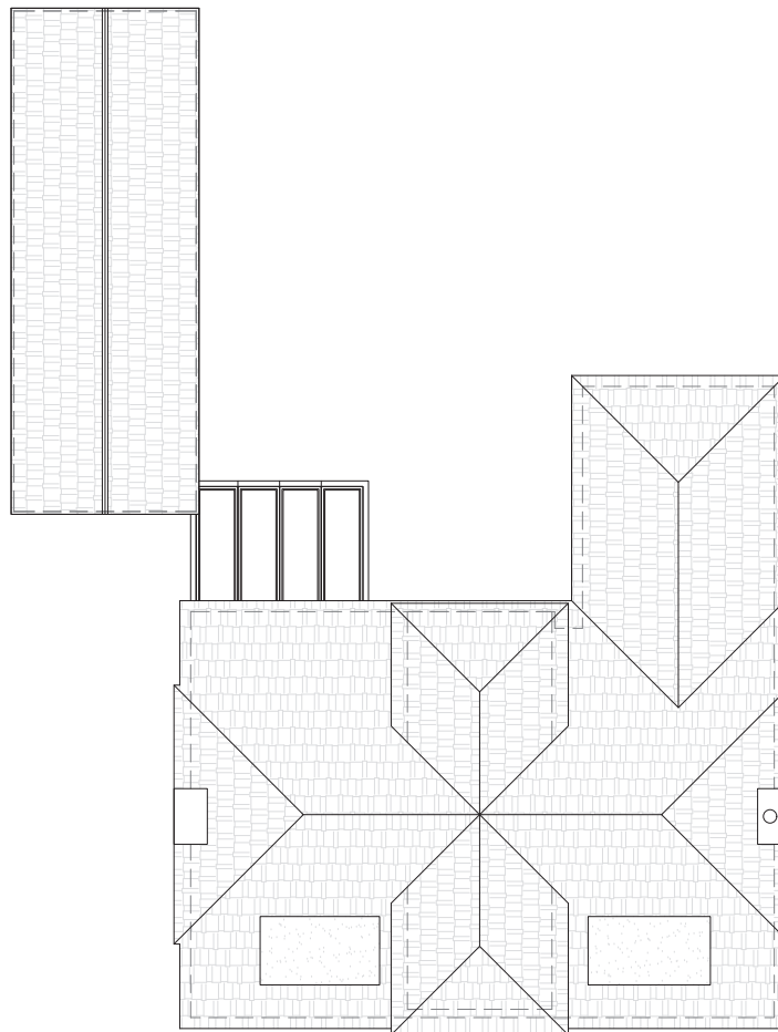
Existing Roof Plan Scale 1:50
