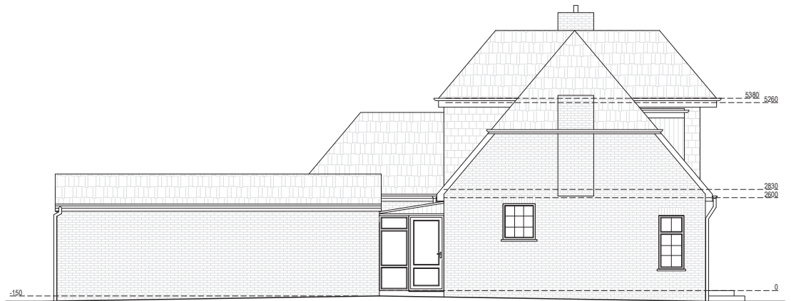
Existing West Elevation Scale 1:50
