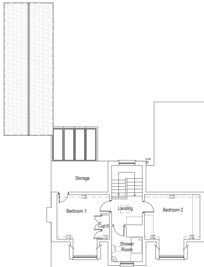
Existing First Floor Plan Scale 1:50 Area ca. 41.11 m 2
