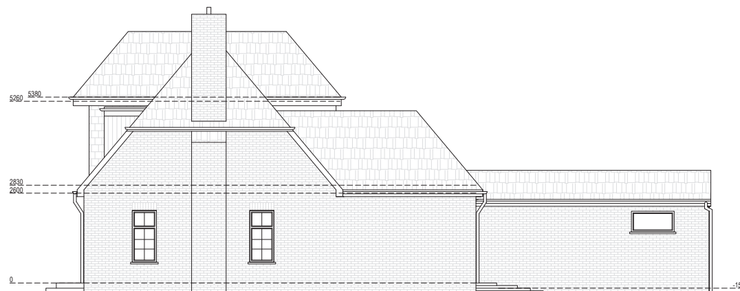
Existing East Elevation Scale 1:50
