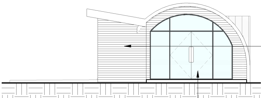
South Elevation 1 : 100
