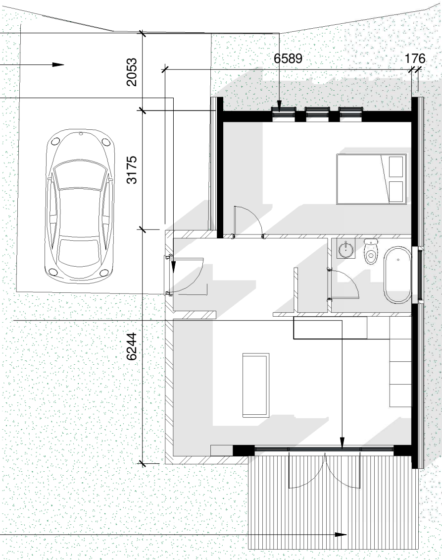
Nissen Hut Ground Floor 1 : 100
