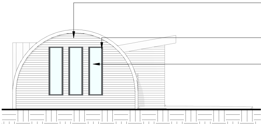
North Elevation 1 : 100
