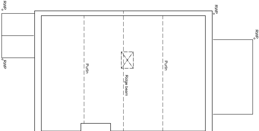
LOFT FLOOR PLAN
