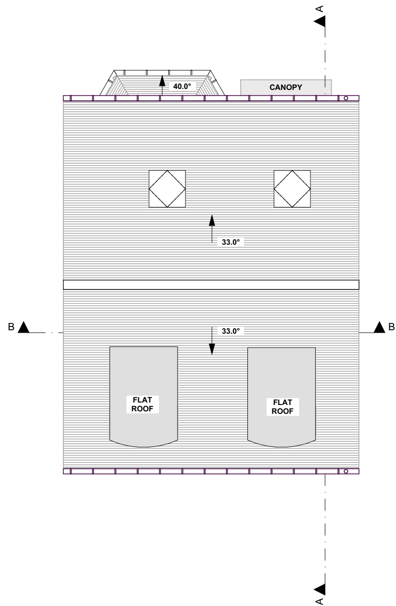
Roof Plan
