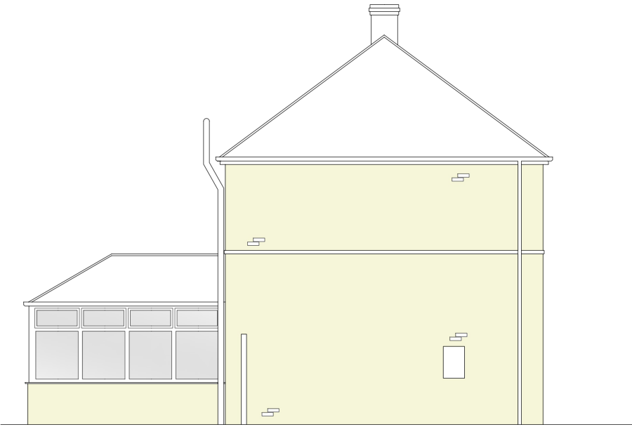
South Elevation Elevation ( Side )
